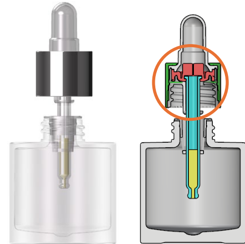
When Opened
